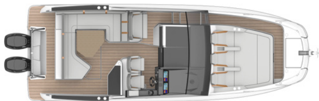
Main deck
